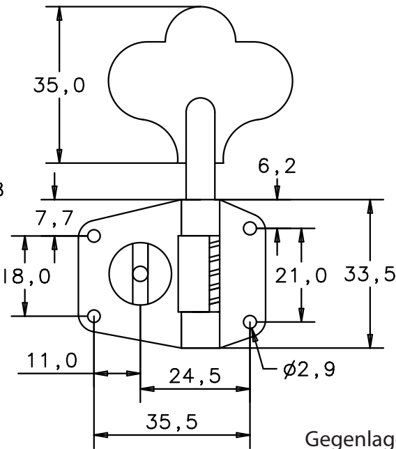
rechte Mechanik right machine head
